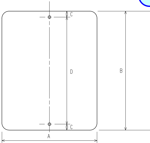
PANELS WITH 2 HOLES DIMENSIONS (INCHES)
