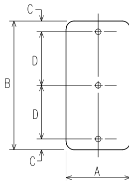
PANELS WITH 3 HOLES DIMENSIONS (INCHES)
