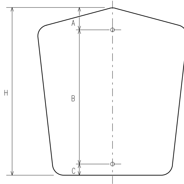
DIMENSIONS (INCHES)
