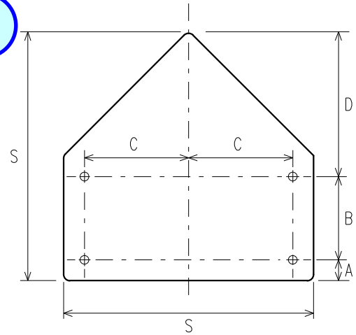
PANELS WITH 4 HOLES DIMENSIONS (INCHES)
