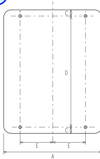
PANELS WITH 4 HOLES DIMENSIONS (INCHES)
