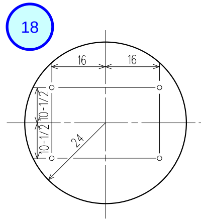
PANELS WITH 4 HOLES
