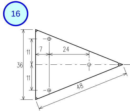
PANELS WITH 3 HOLES
