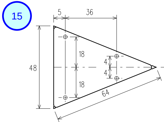
PANELS WITH 4 HOLES
